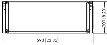
CCL12 cabinet dimensions in mm [inch]
