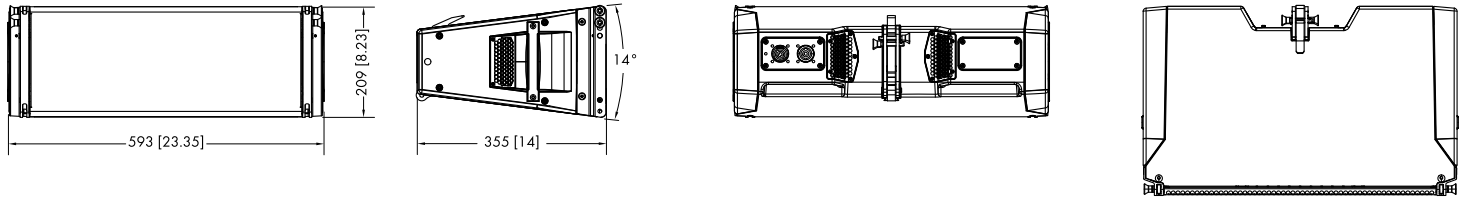
CCL8 cabinet dimensions in mm [inch]
