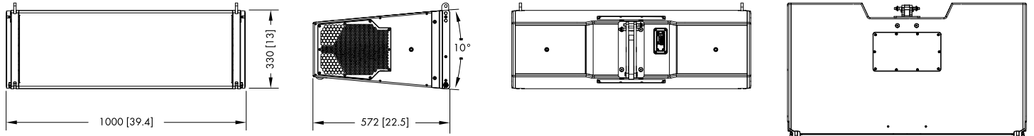
KSL8 cabinet dimensions in mm [inch]
