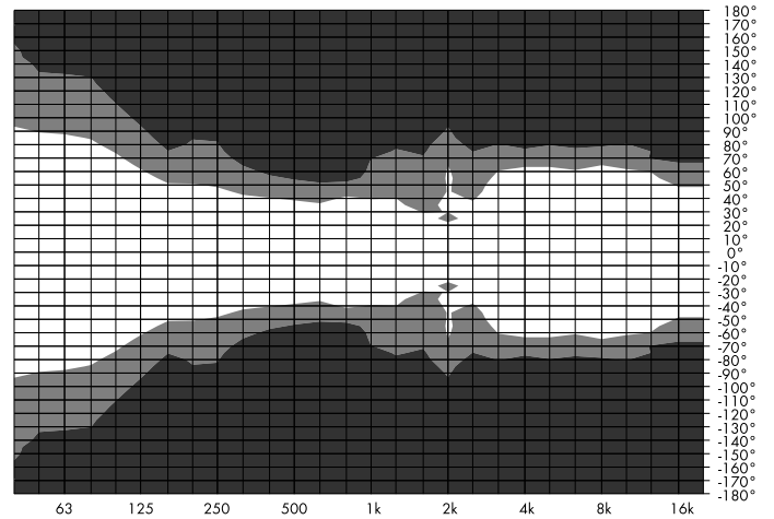
KSLi12 isobar diagram horizontal
