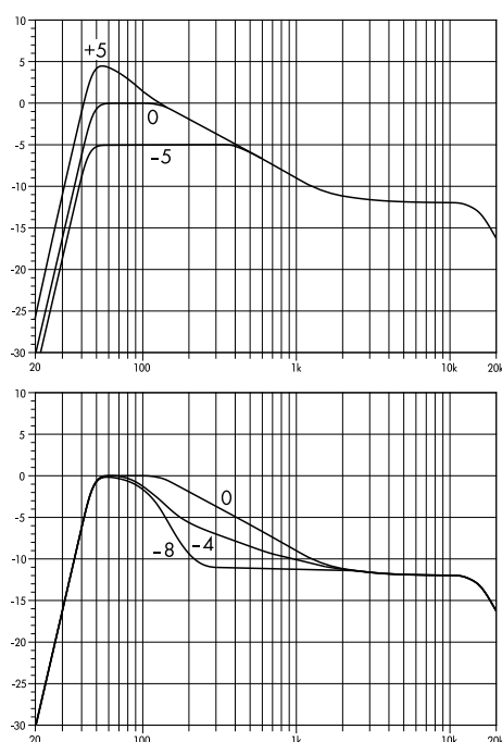
Frequency response correction of the Coupling function for low and low-mid frequency level* *schematic diagram
