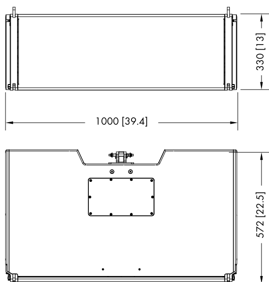
KSli8/KSli12 cabinet dimensions in mm [inch]
