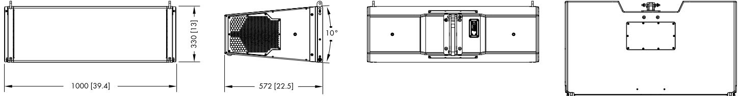
KSLi8 cabinet dimensions in mm [inch]
