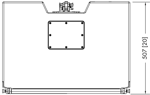
XSL8/XSL12 cabinet dimensions in mm [inch]
