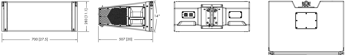
XSL8 cabinet dimensions in mm [inch]
