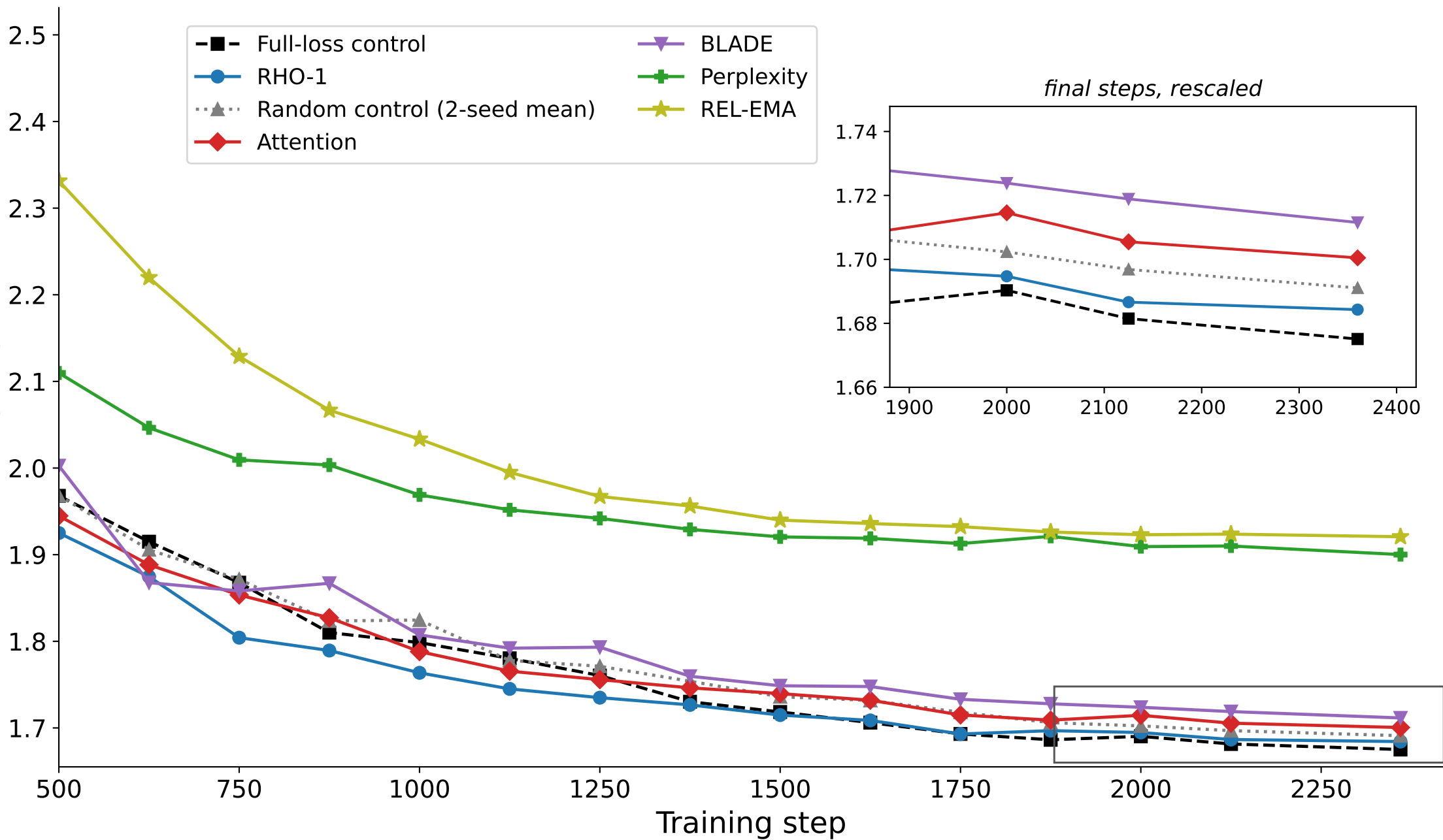
Macro task-loss bits-per-byte (lower is better)
