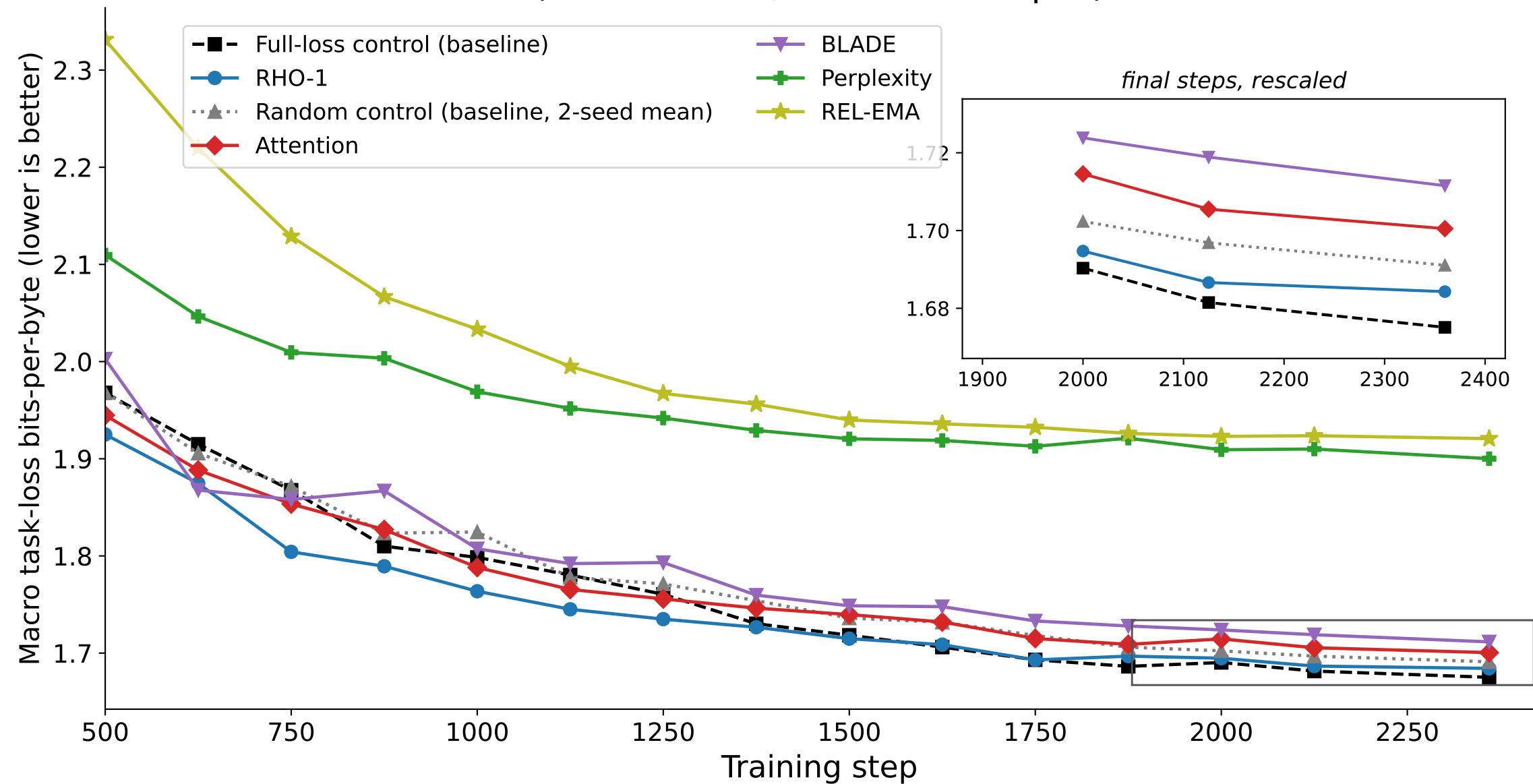
Training curves: macro task-loss bpb by token-filtering arm (370M OLMo2, 10B-token corpus)
