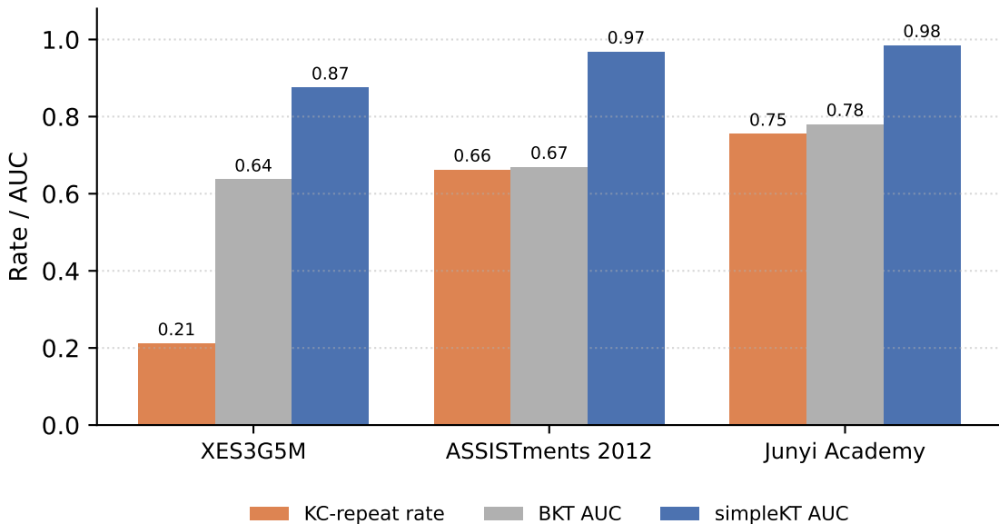
Consecutive KC-repeat rate vs. KT performance
