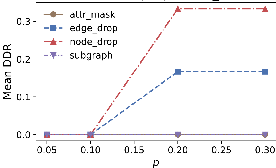
DDR sweep: synthetic_c2
