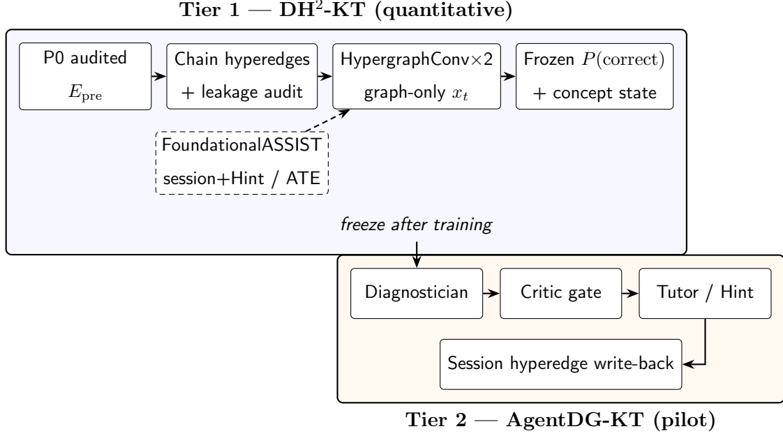
Figure 1: Two-tier DH 2 A-KT architecture. Tier 1 consumes P0’s leakage-audited prerequisite edges as chain hyperedges (solid path; quantitative core on XES3G5M) and optionally FoundationalASSIST session+Hint hyperedges with a limited observational ATE (dashed). After freezing, Tier 2 agents explain and gate those outputs: Diagnostician → Critic → Tutor, with session hyperedge write-back at pilot scale.
