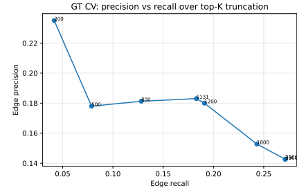
Fig. 5: Edge-level precision and recall of train-only inferred E_{\text{pre}} versus the expert prerequisite annotation on Junyi, across top- K cutoffs K \in \{200, 500, 800, 1131, 1200, 1800, 2500, 3500, 5000\} . The curve plateaus at K \geq 2,500 because the inferred edge pool tops out at 2,152 after DAG audit.
