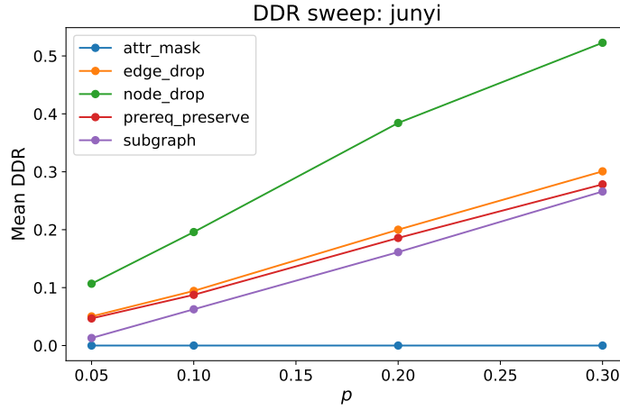
Fig. 6: DDR as a function of perturbation strength p on Junyi Academy for five graph augmentation families: four label-agnostic operators ( attr_mask , subgraph , edge_drop , node_drop ) and one prerequisite-preserving operator ( prereq_preserve ). Each marker plots the mean DDR averaged across nine stochastic runs (three random seeds on each of three train folds). The same ordering holds on ASSISTments 2012 and XES3G5M (Supplementary Figure S2): \text{DDR}(\text{attr\_mask}) = 0 < \text{DDR}(\text{subgraph}) \lesssim \text{DDR}(\text{prereq\_preserve}) < \text{DDR}(\text{edge\_drop}) \approx p < \text{DDR}(\text{node\_drop}) .
