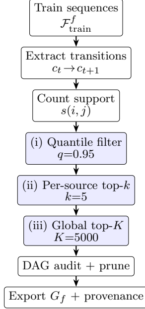
Fig. 4: Train-only prerequisite construction pipeline: temporal transitions are counted on \mathcal{F}_{\text{train}}^f (or optional sample \tilde{\mathcal{Z}}_{\text{tr}}^f ), filtered, cycle-pruned, and exported with provenance fields (Section 3.5).
