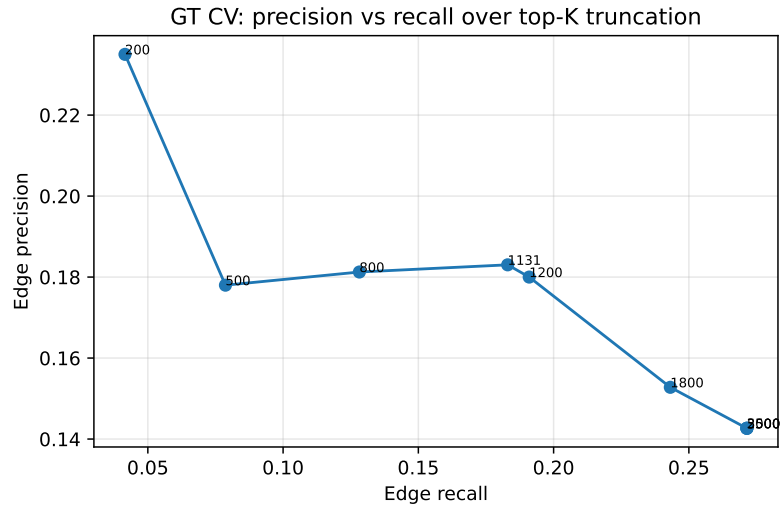
Fig. 4: Edge-level precision and recall of train-only inferred E_{\text{pre}} versus the expert prerequisite annotation on Junyi, across top- K cutoffs K \in \{200, 500, 800, 1131, 1200, 1800, 2500, 3500, 5000\} . The curve plateaus at K \geq 2,500 because the inferred edge pool tops out at 2,152 after DAG audit.
