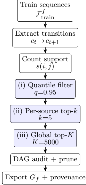
Fig. 4: Train-only prerequisite construction pipeline: temporal transitions are counted on \mathcal{F}_{\text{train}}^f (or optional sample \tilde{\mathcal{L}}_{\text{tr}}^f ), filtered, cycle-pruned, and exported with provenance fields (Section ??).
