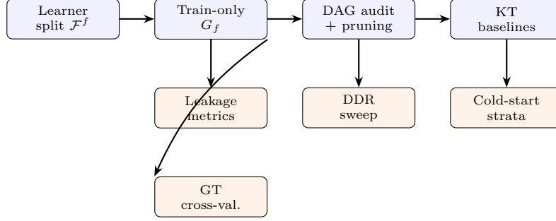
Fig. 2: Research framework connecting protocol modules (Section ??) and experiment tracks (Section ??). Fold-conditioned provenance, DAG repair, structural diagnostics decoupled from AUC, and optional expert cross-validation are the core audit outputs.
