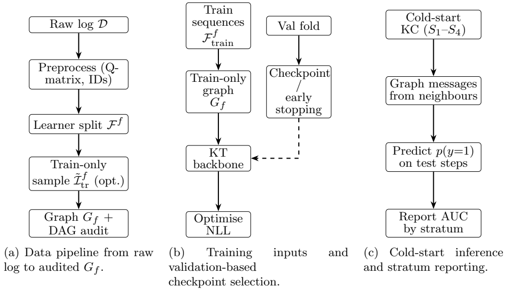
Fig. 3: End-to-end protocol plumbing: (a) data preparation and fold-conditioned graph construction, (b) training with a train-only graph and validation-based checkpoint selection, and (c) cold-start knowledge-component evaluation with stratum-specific reporting (Section 4.8).
