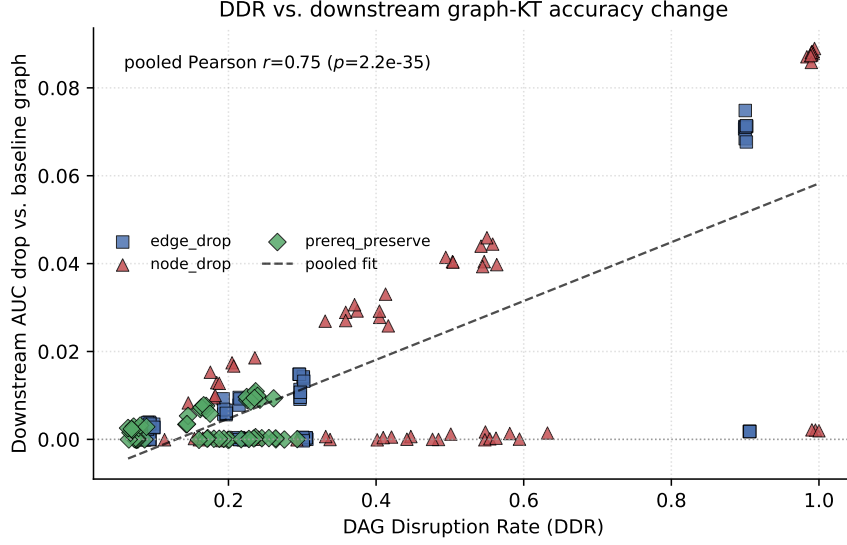
Fig. 9: Supplementary Figure S3. Downstream graph-KT sensitivity to prerequisite-graph disruption on ASSISTments 2012 and XES3G5M (DGEKT and GKT cells). Each point is one fold/operator/strength run; the vertical axis is AUC drop relative to the unperturbed train-only graph. The burned-in annotation r \approx 0.75 is the global pooled Pearson correlation across both datasets and both models ( n=186 ), not the XES3G5M/GKT-only correlation ( r \approx 0.99 with anchors, n=66 ; r \approx 0.95 on the p \leq 0.3 core, n=54 ).
