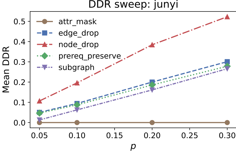
Fig. 5: DDR as a function of perturbation strength p on Junyi Academy for five graph augmentation families: four label-agnostic operators ( attr_mask , subgraph , edge_drop , node_drop ) and one prerequisite-preserving operator ( prereq_preserve ). Each marker plots the mean DDR averaged across nine stochastic runs (three random seeds on each of three train folds). The same ordering holds on ASSISTments 2012 and XES3G5M (Supplementary Figure S2): \text{DDR}(\text{attr\_mask}) = 0 < \text{DDR}(\text{subgraph}) \lesssim \text{DDR}(\text{prereq\_preserve}) < \text{DDR}(\text{edge\_drop}) \approx p < \text{DDR}(\text{node\_drop}) .
