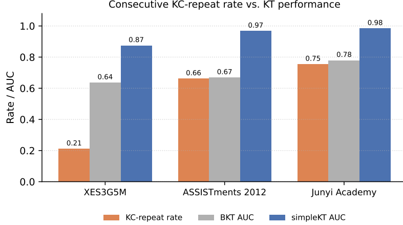
Fig. 8: Consecutive KC-repeat rate against simpleKT AUC across the three public benchmarks.
