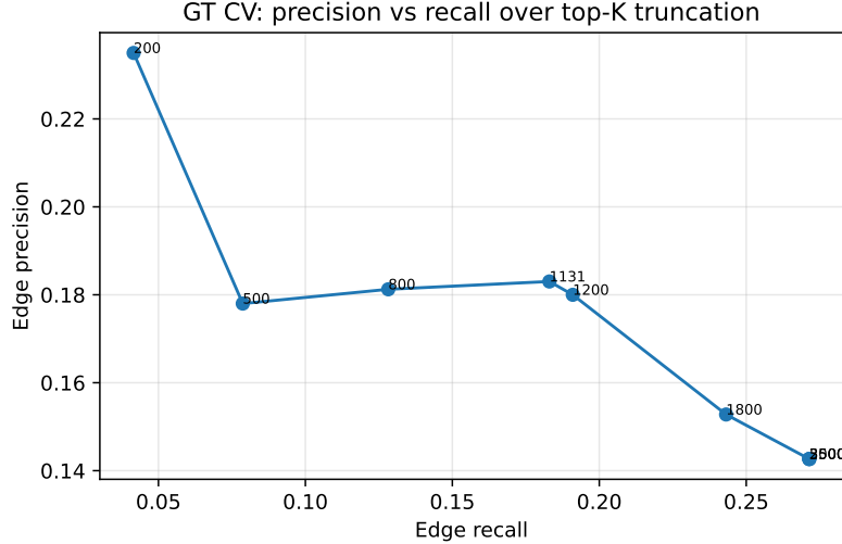
Fig. 7: Edge-level precision and recall of train-only inferred E_{\text{pre}} versus the expert prerequisite annotation on Junyi, across top- K cutoffs K \in \{200, 500, 800, 1131, 1200, 1800, 2500, 3500, 5000\} . The curve plateaus at K \geq 2,500 because the inferred edge pool tops out at 2,152 after DAG audit.
