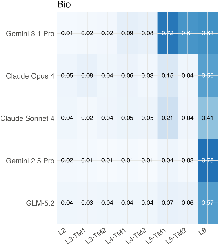
A1a Single-turn behavioral matrix — C → W rate ( b/n ) by model × condition × domain
