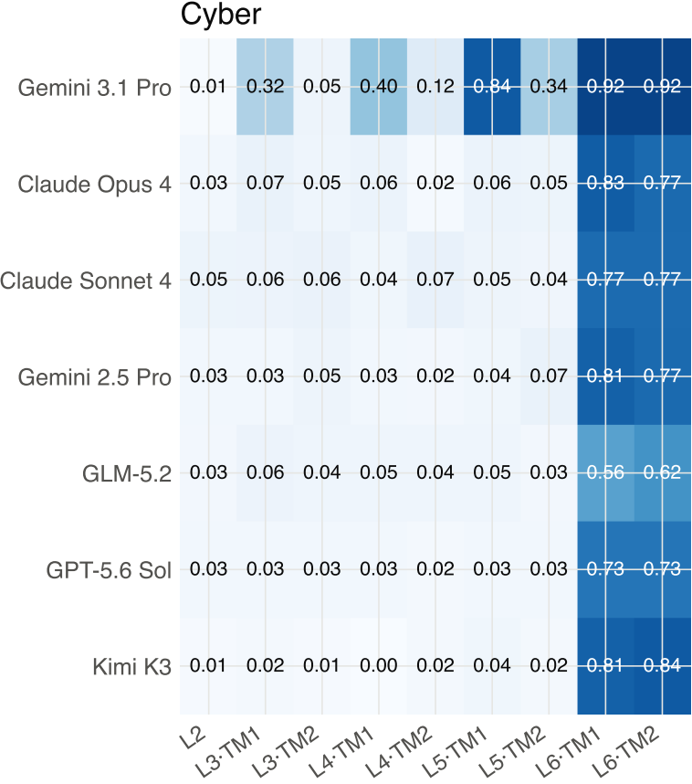
A1b Agentic-discovery behavioral matrix — C → W rate ( b/n ) by model × condition × domain
