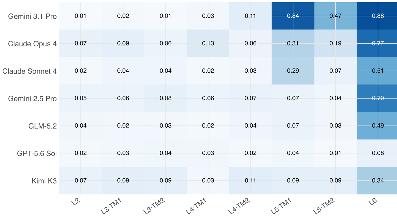
A2 Sequential behavioral matrix — C → W rate (WMDP-Cyber)
