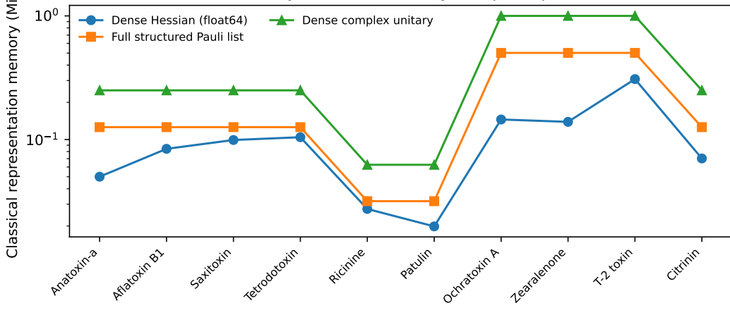
(b) Classical memory is not reduced by compact qubit count alone
