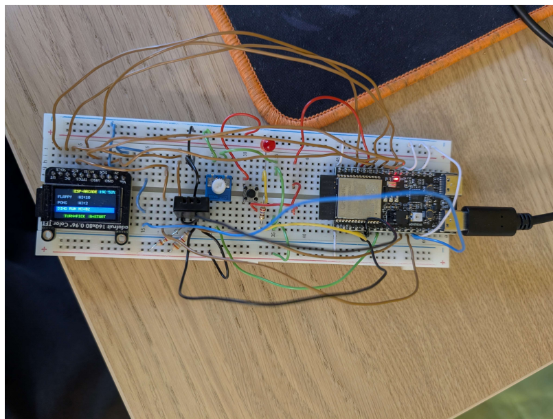
Figura 2: Final breadboard implementation
