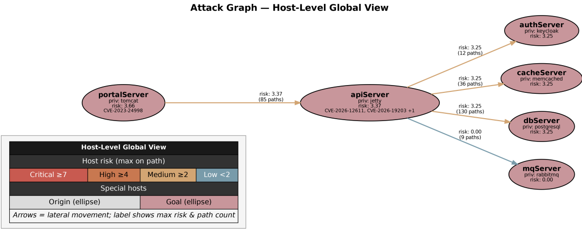
Figure 26: Scenario 3 host-level summary graph: deep lateral movement from the DMZ to the API server, which fans out into the identity and data tiers.
