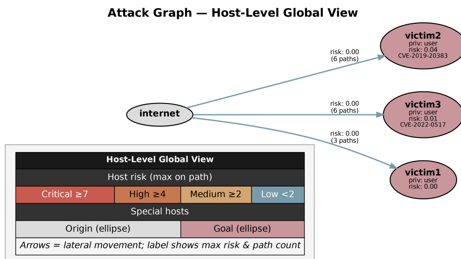
Figure 21: Scenario 1 host-level summary graph: each victim is reached directly from the internet, annotated with its worst-case path risk and exploited CVEs.
