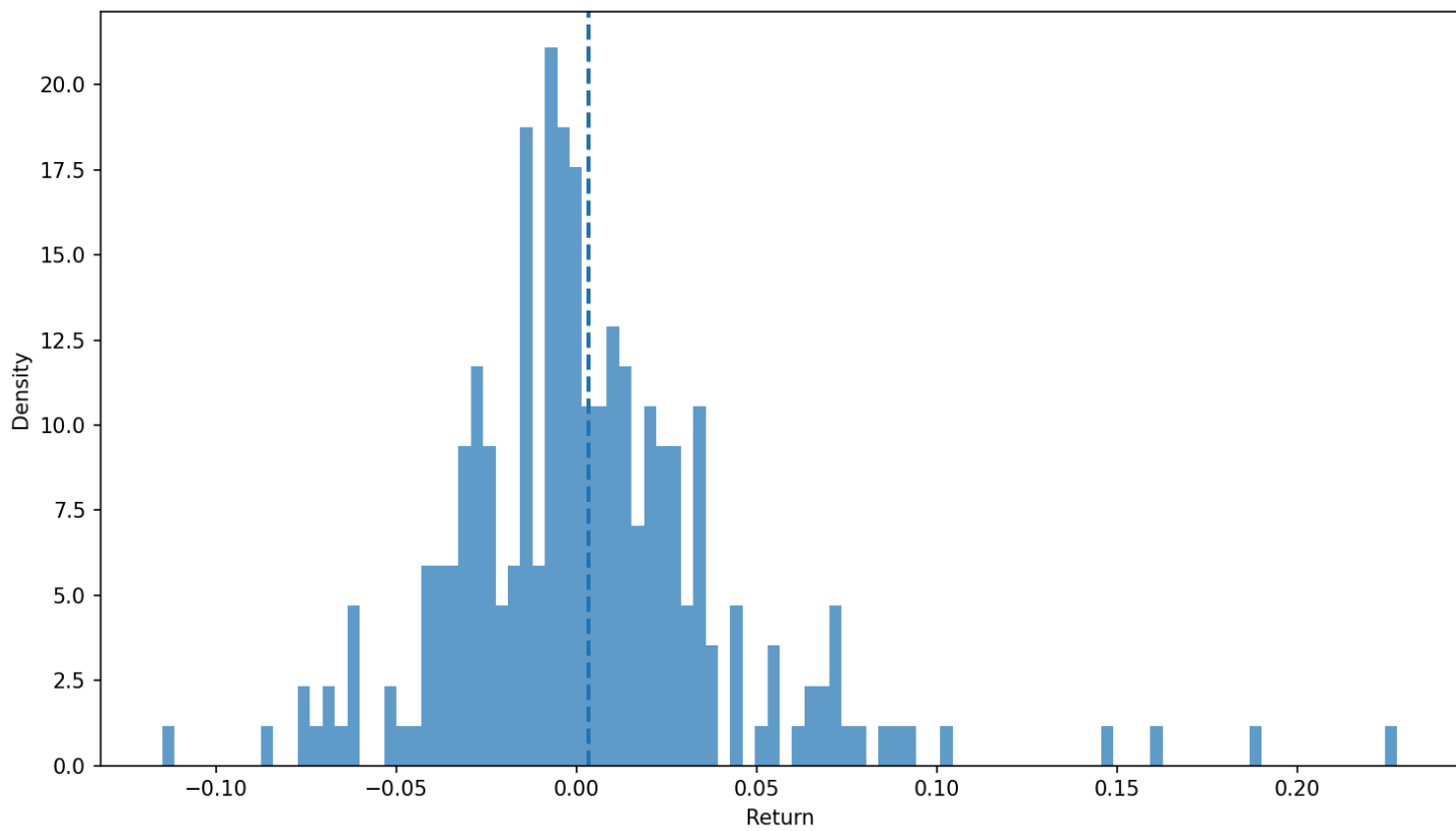
INTC — Return Distribution
