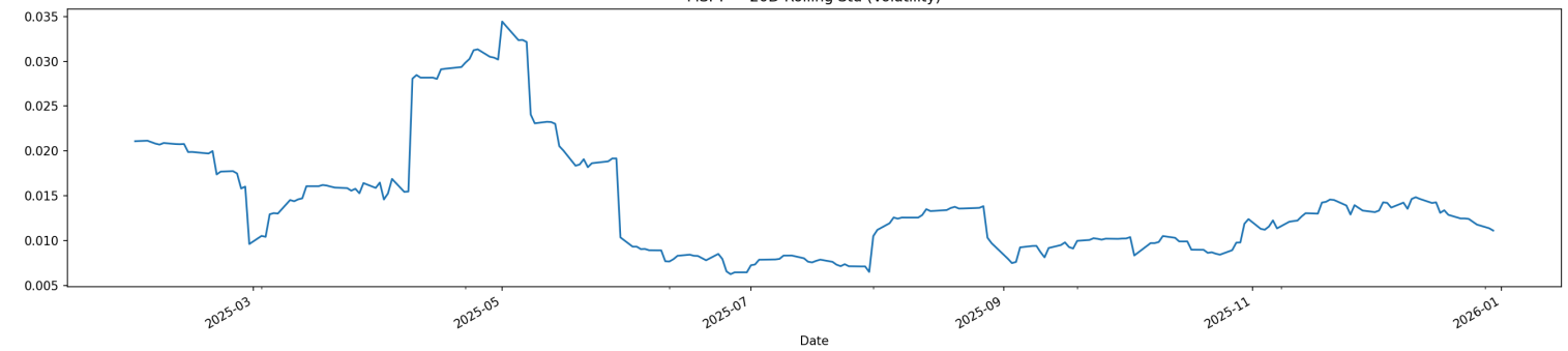
MSFT — 20D Rolling Std (Volatility)
