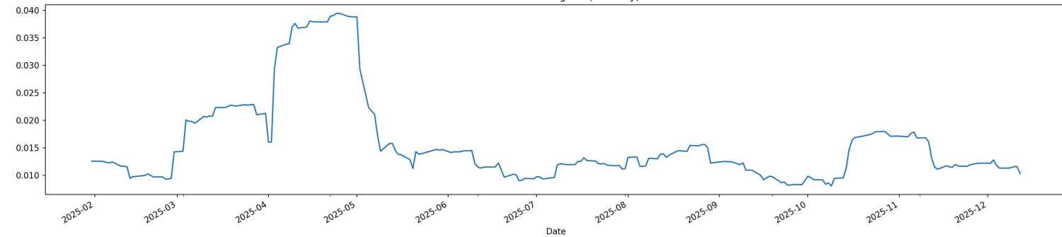
BAC — 20D Rolling Std (Volatility)
