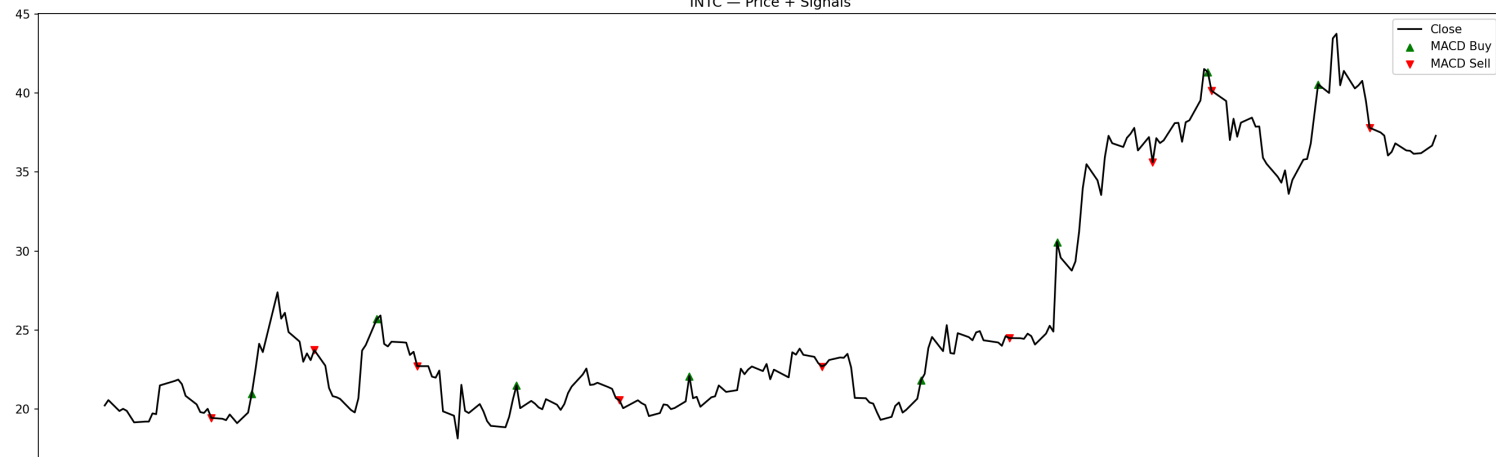
INTC — Price + Signals
