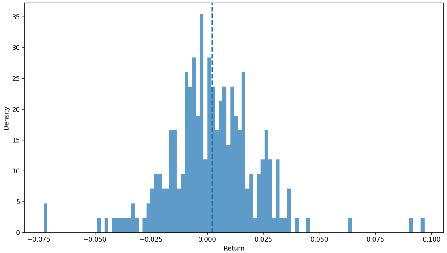
GOOGL — Return Distribution
