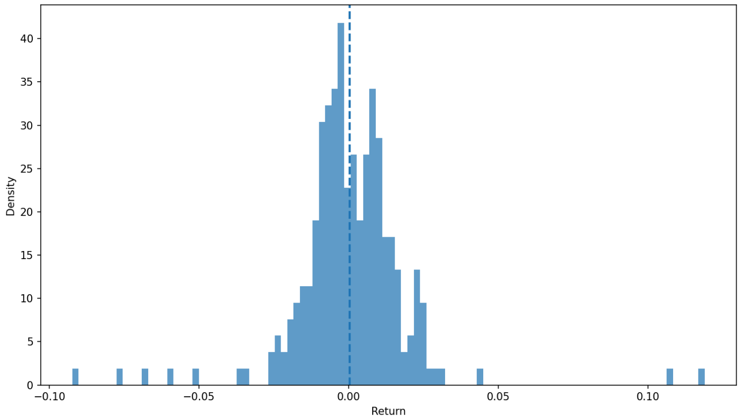
DIS — Return Distribution
