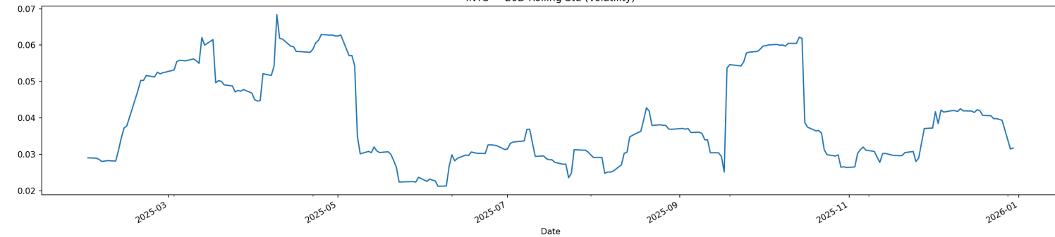
INTC — 20D Rolling Std (Volatility)
