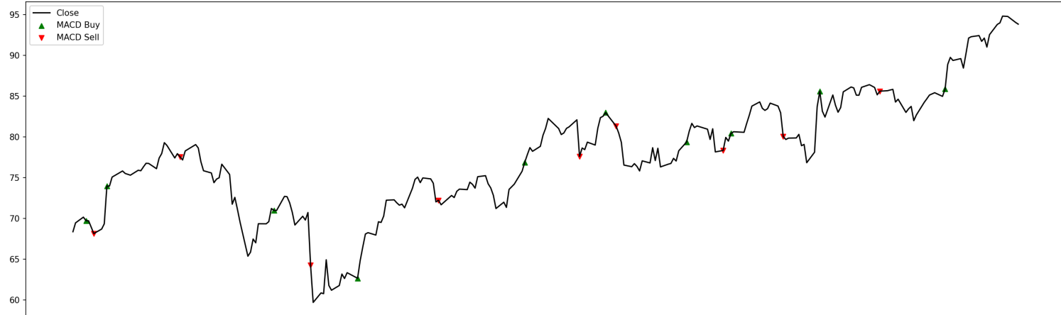
WFC — Price + Signals
