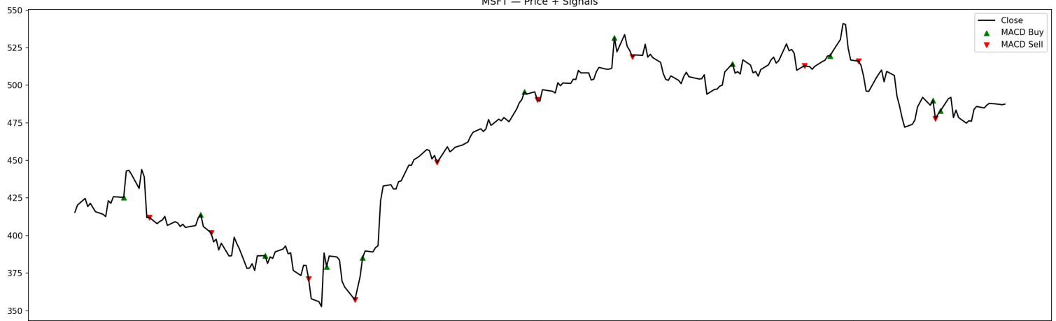
MSFT — Price + Signals
