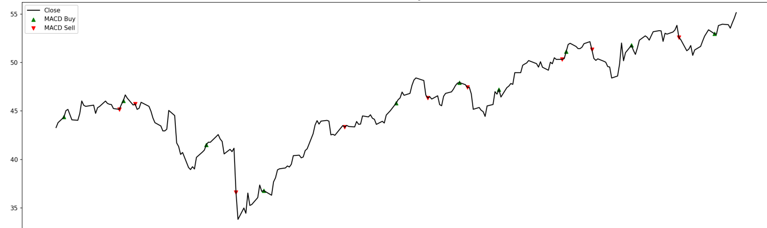
BAC — Price + Signals
