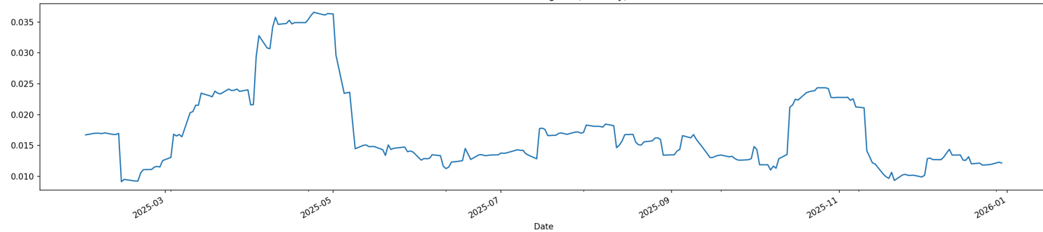
WFC — 20D Rolling Std (Volatility)
