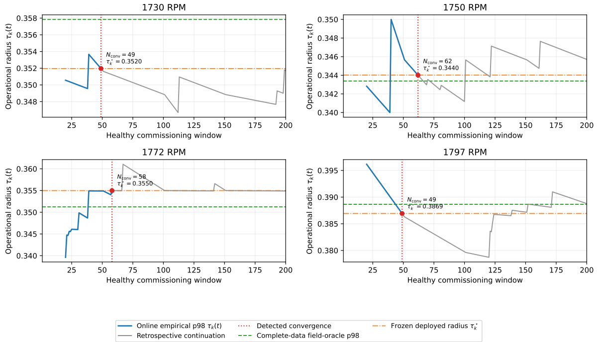
Figure 3: Sequential estimation of the empirical p98 operational radius during CWRU commissioning. For each operating condition, the blue segment shows the online estimate \tau_k(t) = \hat{Q}_{k,t}(0.98) until the convergence criterion is satisfied. The red dotted line marks the declared convergence point, at which the operational radius is frozen and active monitoring begins. The gray segment is a retrospective continuation obtained by incorporating additional observations known from the benchmark to be healthy; it is shown only to characterize the subsequent behaviour of the estimator and is not used to modify the deployed decision boundary. The horizontal dashed line indicates the complete-data field-oracle p98 reference.
