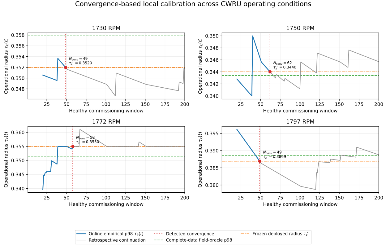
FIGURE 1 Sequential estimation of the empirical p98 operational radius during CWRU commissioning. For each operating condition, the blue segment shows the online estimate defined in Eq. (3), \tau_k(t) = \widehat{Q}_{k,t}(0.98) , until the convergence criterion is satisfied. The red dotted line marks the declared convergence point, at which the operational radius is frozen and active monitoring begins. The gray segment is a retrospective continuation obtained by incorporating additional observations known from the benchmark to be healthy; it is shown only to characterize the subsequent behaviour of the estimator and is not used to modify the deployed operational radius. The horizontal dashed line indicates the complete-data field-oracle reference defined in Eq. (5).
