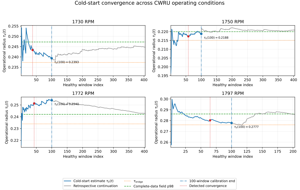
Figure 5: Cold-start convergence and retrospective evolution of the local operational radius across the four CWRU operating conditions. The blue segment shows the sequential radius estimate during the 100-window calibration interval used by the deployed detector. The red dotted line marks the detected convergence index, and the blue dash-dotted line marks the end of the prescribed cold-start interval. The gray segment is a retrospective cumulative estimate obtained by continuing to incorporate the remaining known-healthy observations; it is shown only to characterize the subsequent evolution of the estimator and is not used to update the deployed decision boundary. Horizontal lines indicate the transferred standardized radius \tau_{bridge} and the complete-data field p98 reference.
