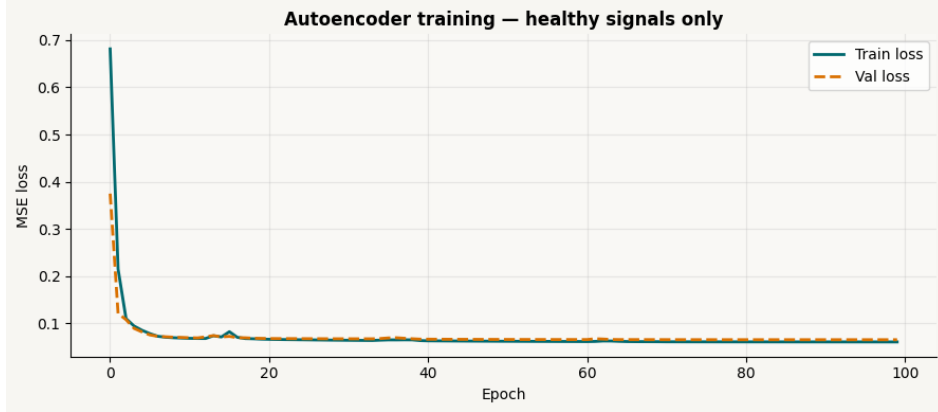
Figure 2: Training and validation loss of the healthy-only Conv1D autoencoder used as the shared nominal representation.
