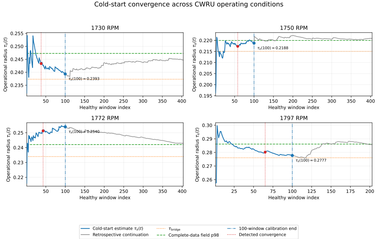
Figure 4: Cold-start convergence and retrospective evolution of the standardized bridge radius across the four CWRU operating conditions. The blue segment shows the sequential estimate \tau_{\text{bridge},k}(t) = \mu_k(t) + z_{\text{MC}}\sigma_k(t) during the prescribed 100-window calibration interval. The red dotted line marks the detected convergence index, and the blue dash-dotted line marks the end of the calibration interval. The gray segment is a retrospective continuation using the remaining known-healthy observations and is not used by the deployed detector. The horizontal orange line indicates the bridge radius computed from the complete healthy residual mean and standard deviation, whereas the horizontal green line indicates the complete-data empirical p98 field-oracle reference.
