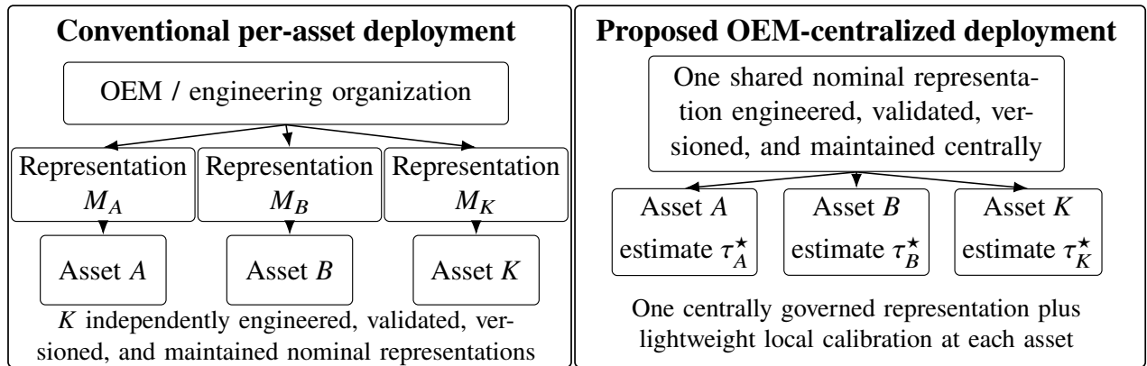
FIGURE 1 Conventional fleet deployment requires engineering, validating, versioning and maintaining an independent nominal representation for each monitored asset. The proposed deployment architecture instead distributes one shared nominal representation unchanged across the fleet, while each asset estimates only its local operational radius during commissioning. The NASA IMS experiments demonstrate that these locally estimated radii differ substantially between physical assets, despite using the same representation, the same target nominal coverage, and the same convergence criterion.
