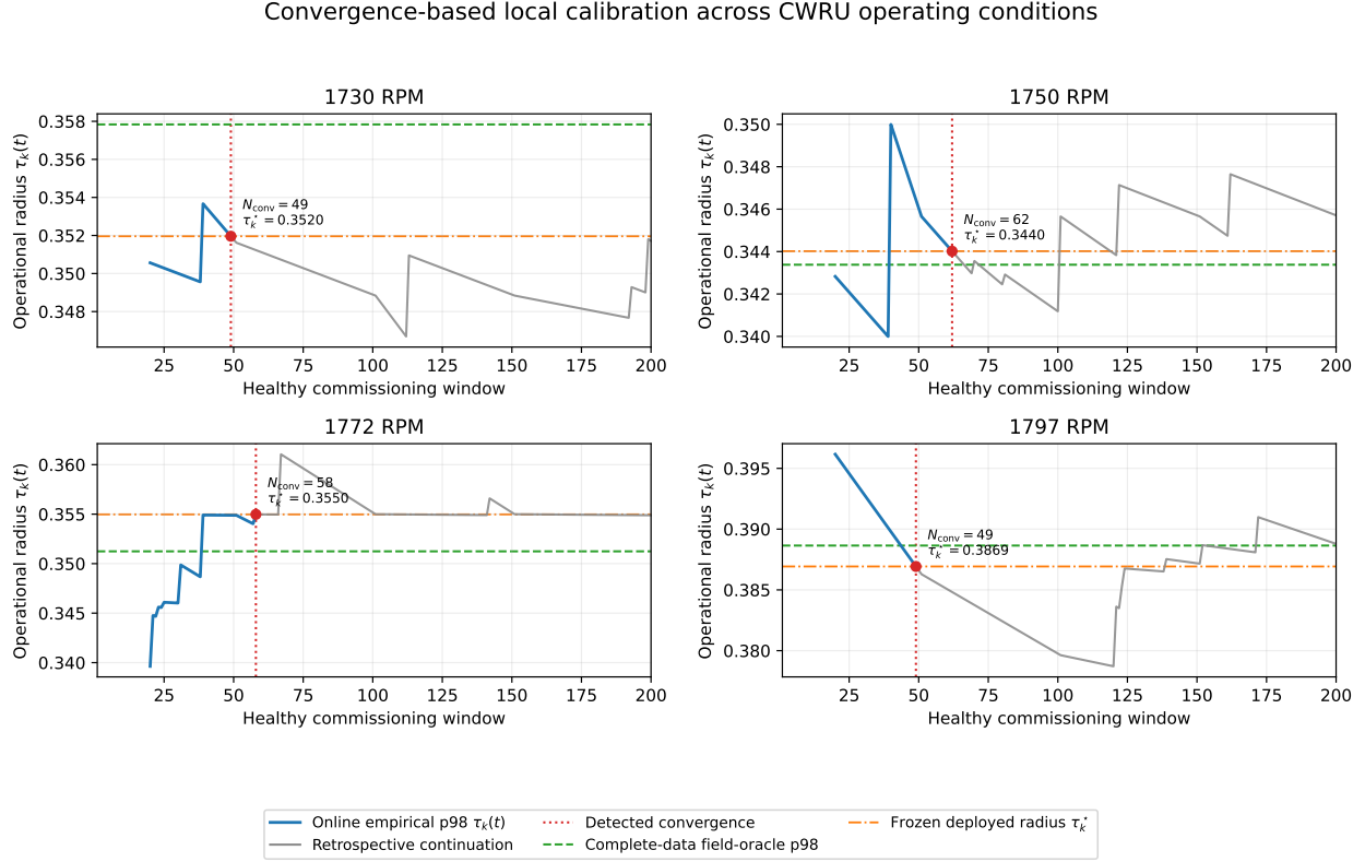
FIGURE 2 Sequential estimation of the empirical p98 operational radius during CWRU commissioning. For each operating condition, the blue segment shows the online estimate defined in Eq. (3), \tau_k(t) = \widehat{Q}_{k,t}(0.98) , until the convergence criterion is satisfied. The red dotted line marks the declared convergence point, at which the operational radius is frozen and active monitoring begins. The gray segment is a retrospective continuation obtained by incorporating additional observations known from the benchmark to be healthy; it is shown only to characterize the subsequent behaviour of the estimator and is not used to modify the deployed operational radius. The horizontal dashed line indicates the complete-data field-oracle reference defined in Eq. (5).
