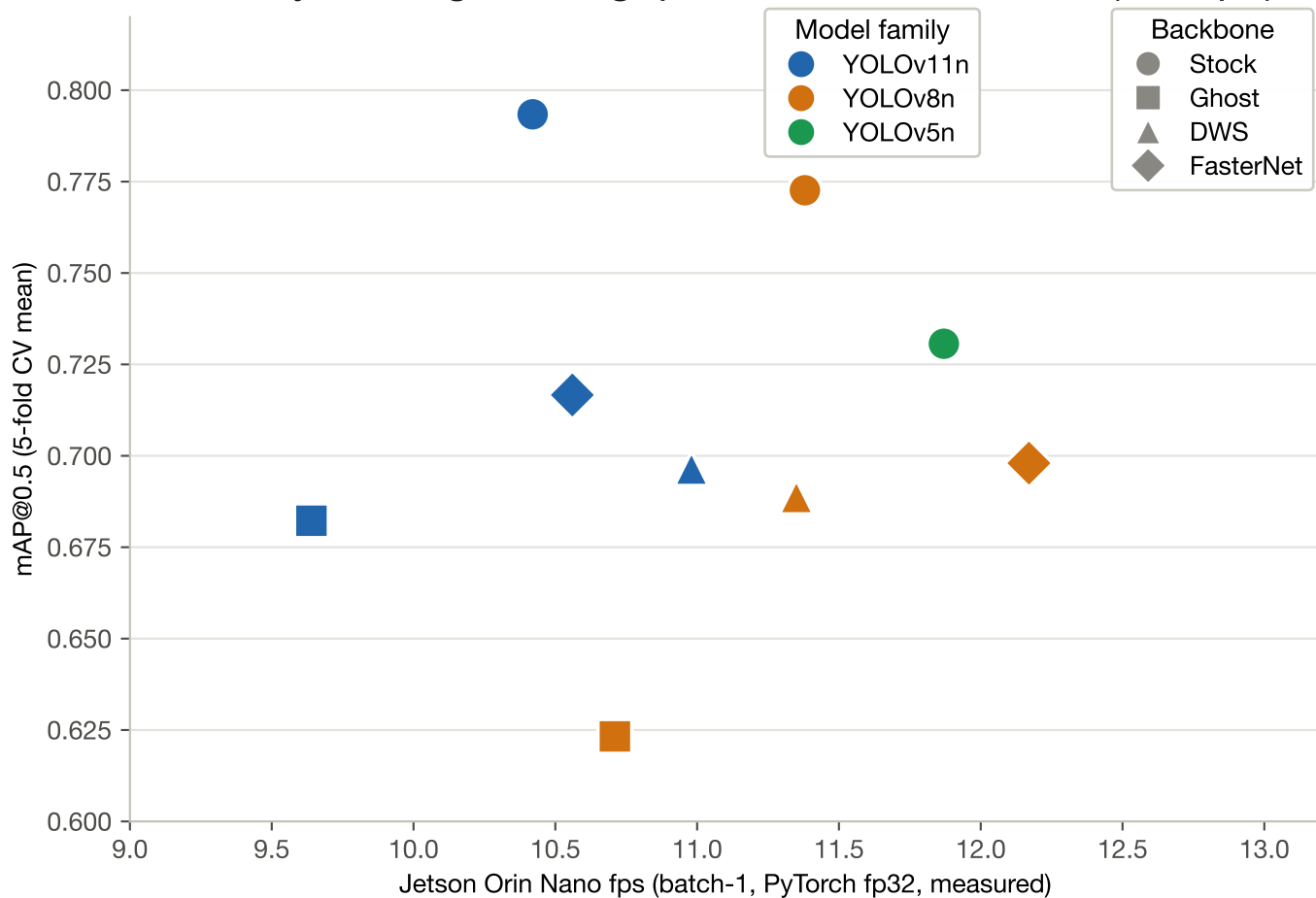
Accuracy vs. edge throughput across backbones (1280px)
