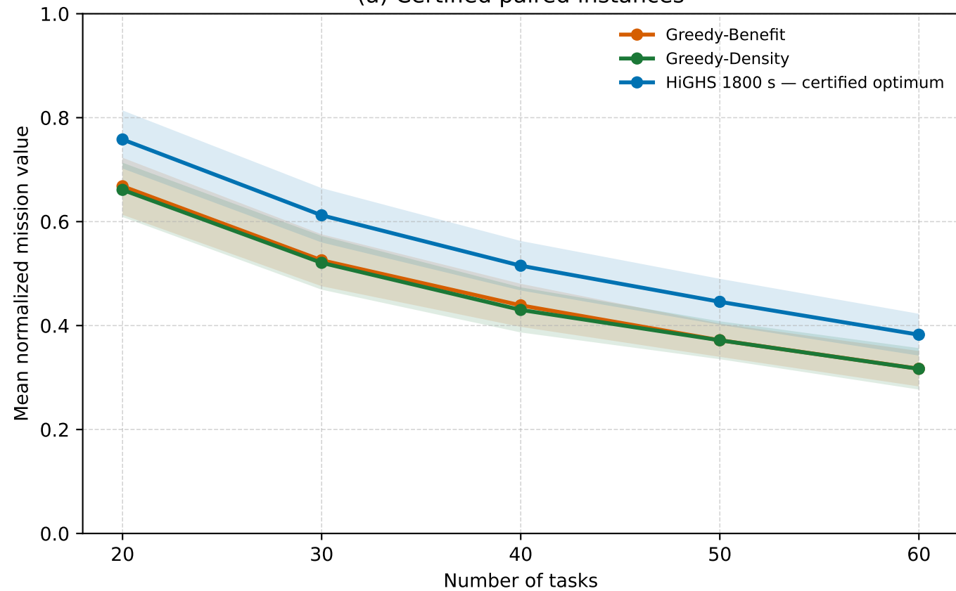
(a) Certified paired instances
