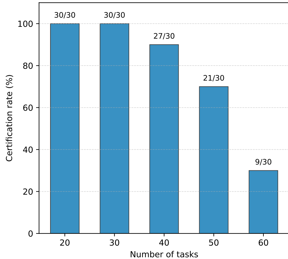
(b) Optimality certification at 1800 s
