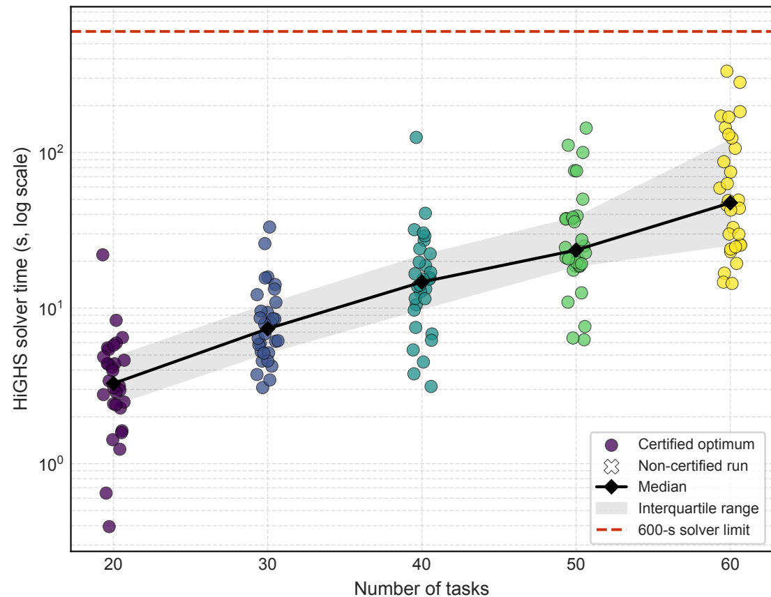
(a) HiGHS computational effort
