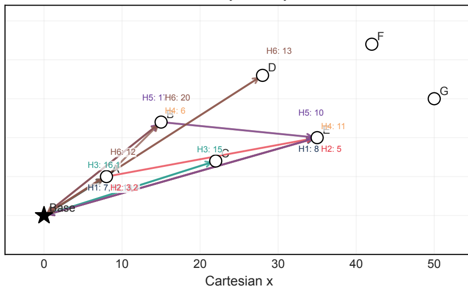
Greedy-Density
