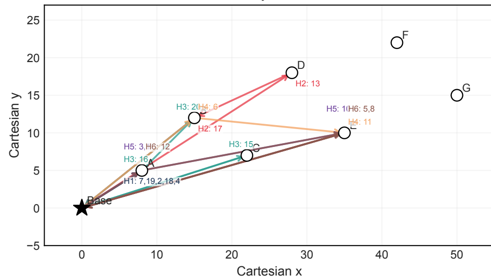
Greedy-Benefit
