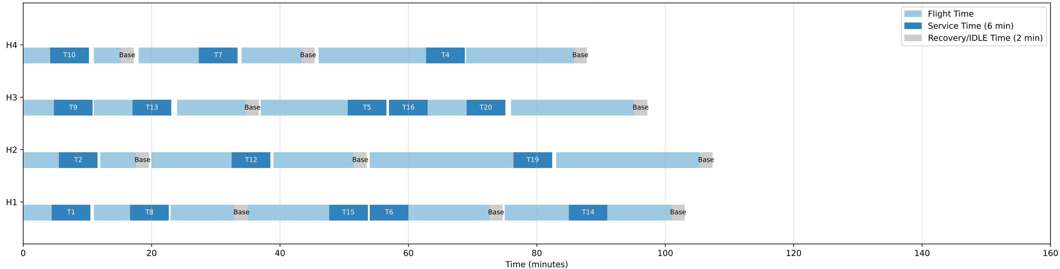
Gantt Chart - Proposed Greedy TTAP
