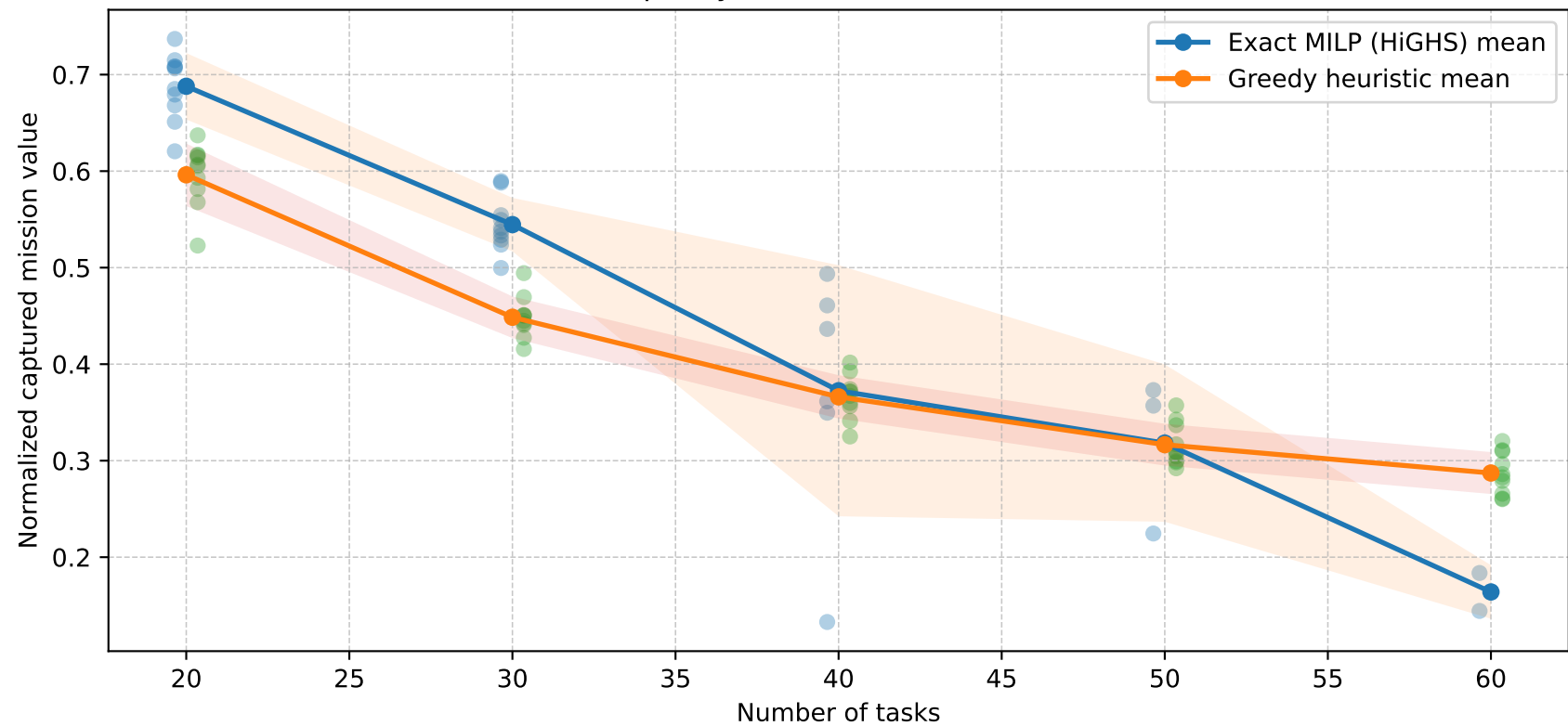
Solution quality across scaled TTAP instances
