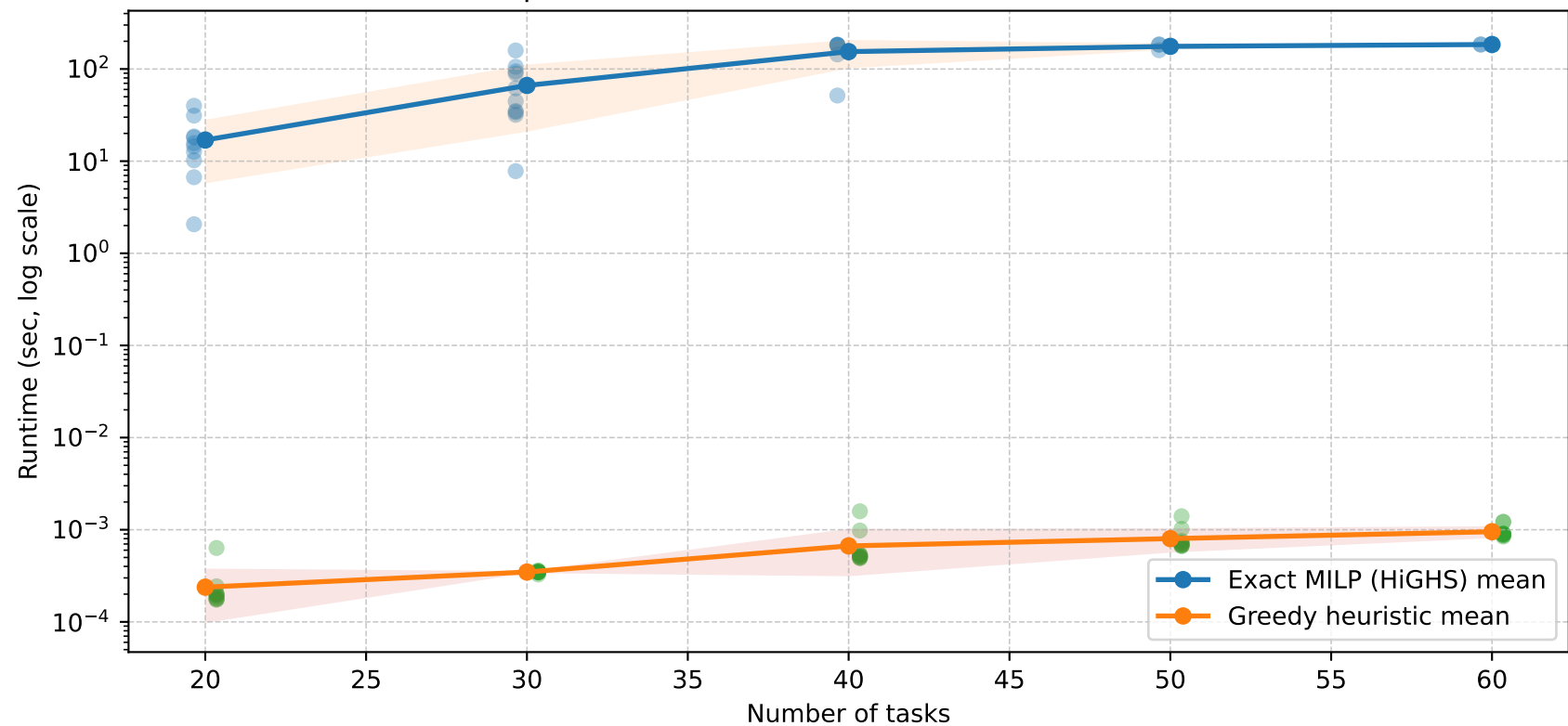
Computational runtime across scaled TTAP instances
