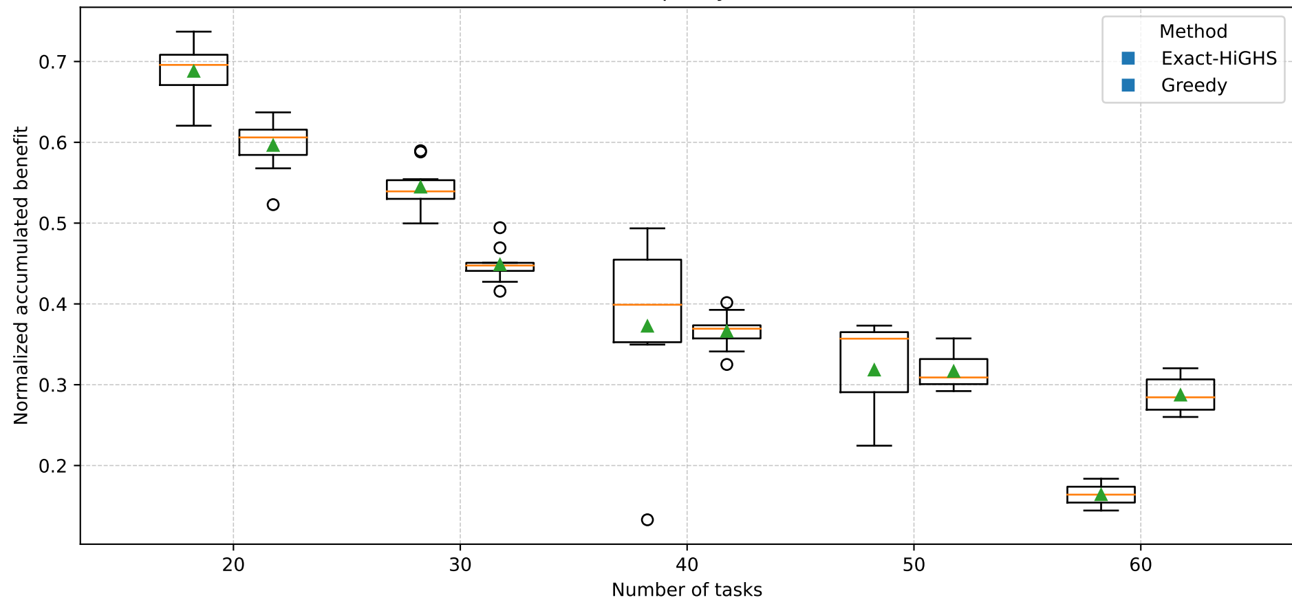
Distribution of solution quality across TTAP instances
