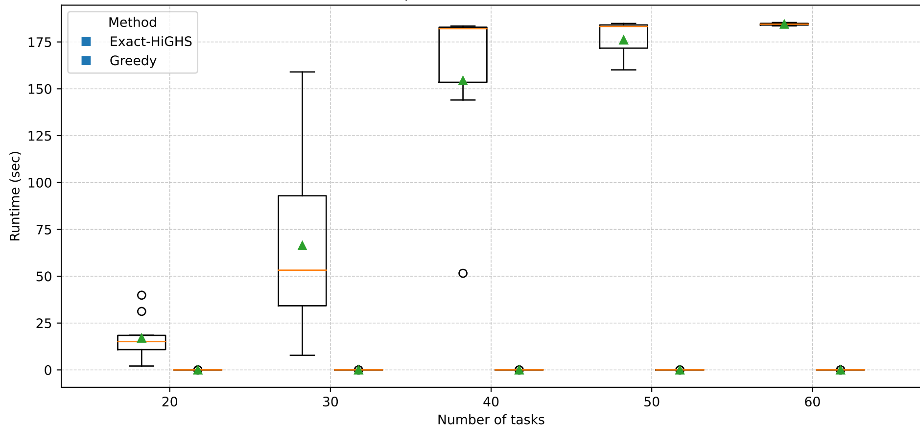
Distribution of computational runtime across TTAP instances
