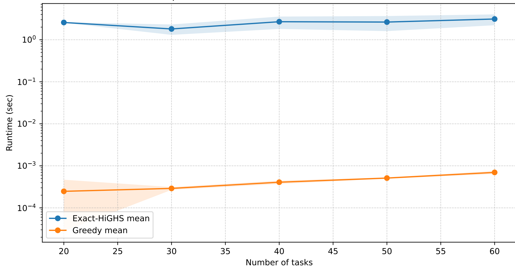
Computational runtime across scaled TTAP instances
