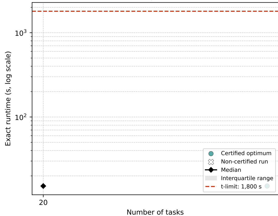
(a) Exact computational effort
