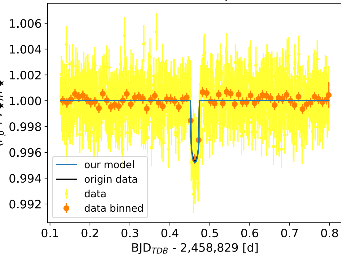
Phase curve at \lambda = 0.7 \mu\text{m} with FGS1
