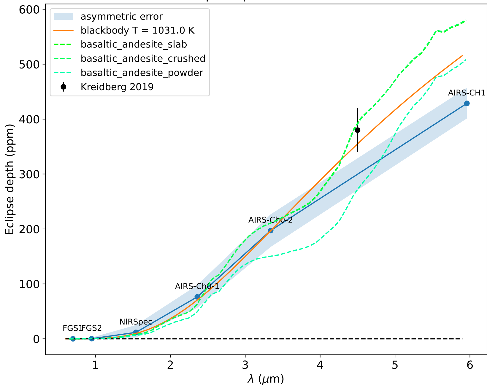
Eclipse depths for LHS3844b
