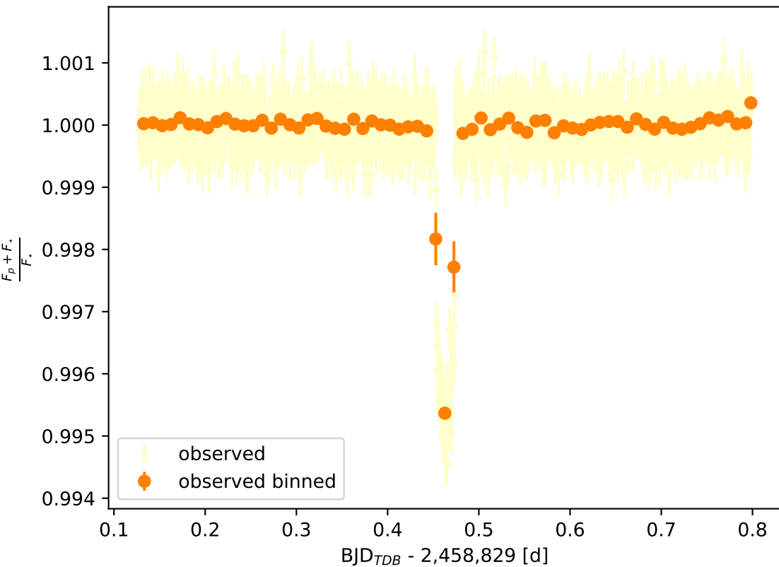
Phase curve at \lambda = 1.54 \mu\text{m} with NIRSpec
