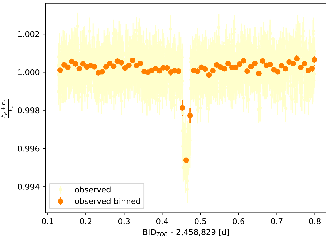
Phase curve at \lambda = 5.96 \mu\text{m} with AIRS-CH1
