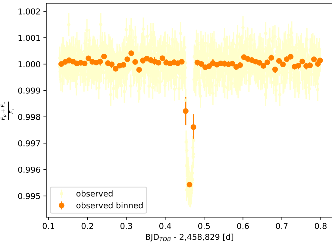
Phase curve at \lambda = 2.36 \mu\text{m} with AIRS-Ch0-1
