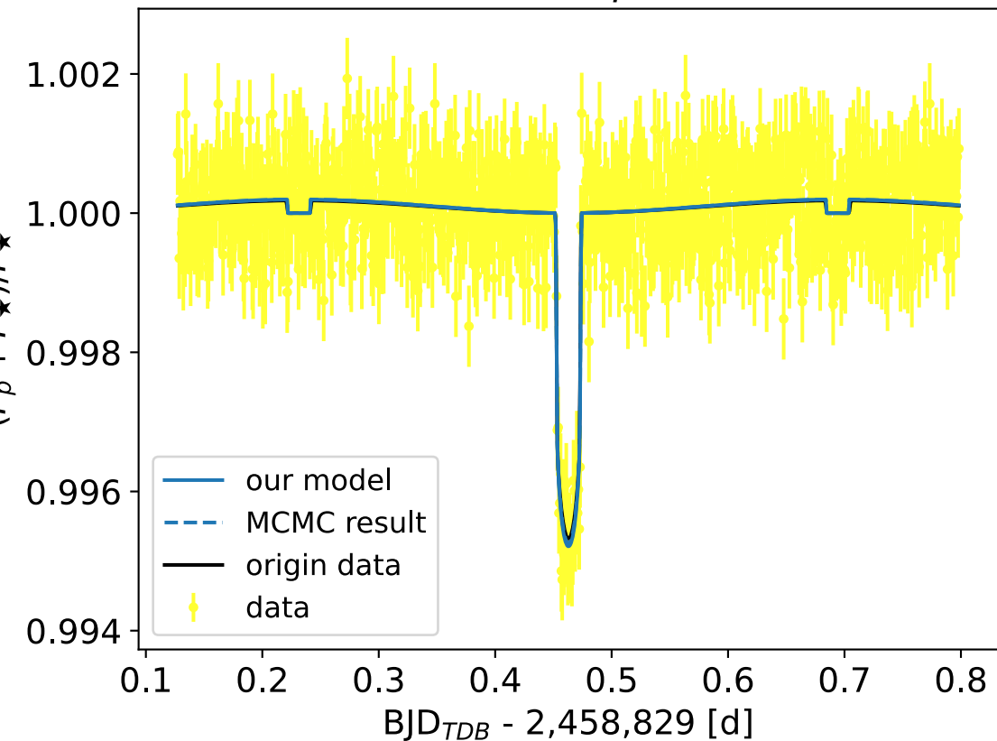
Phase curve at \lambda = 3.34 \mu\text{m} with AIRS-Ch0-2
