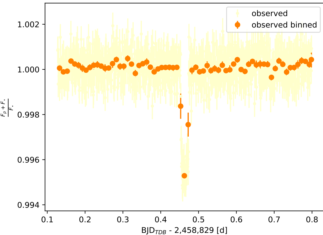
Phase curve at \lambda = 3.34 \mu\text{m} with AIRS-Ch0-2
