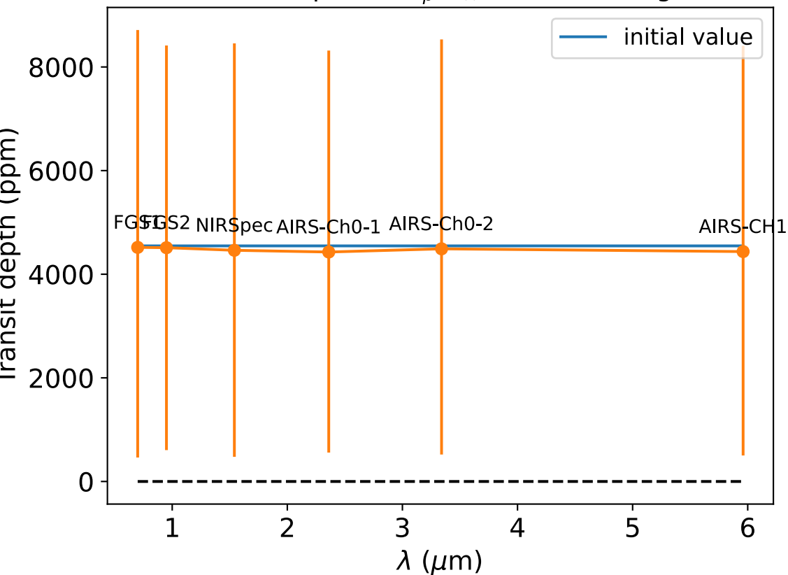
Transit depth = (R_p/R_\star)^2 vs wavelength
