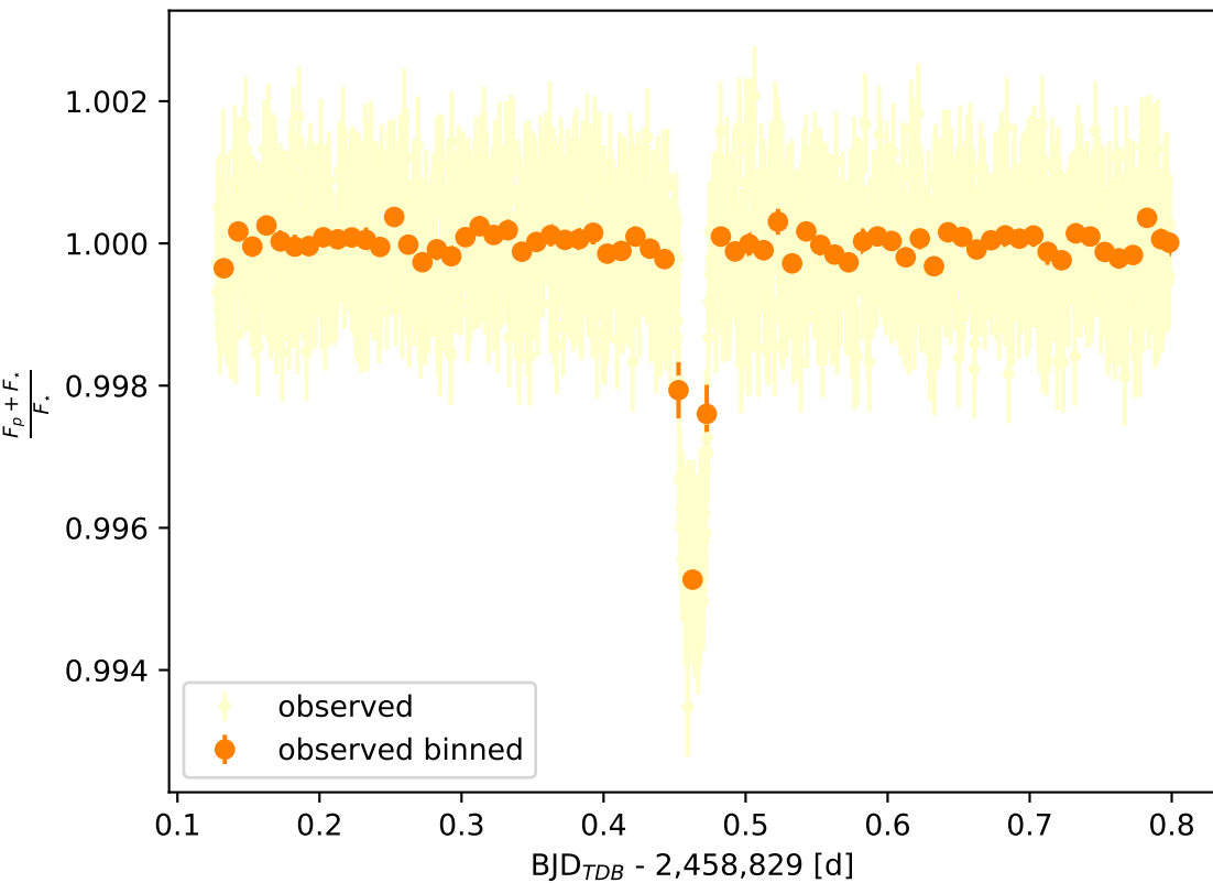
Phase curve at \lambda = 0.95 \mu\text{m} with FGS2
