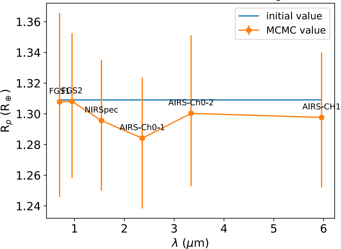
Radius of LHS 3844 b vs wavelength
