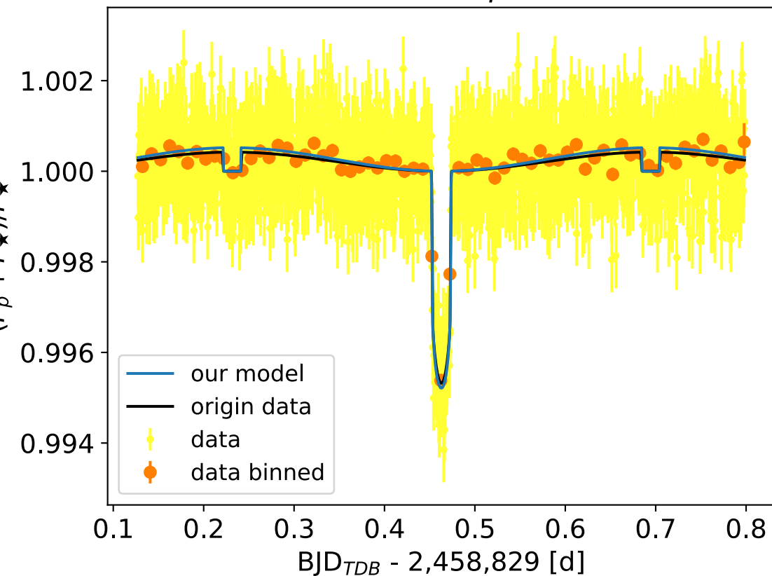
Phase curve at \lambda = 5.96 \mu\text{m} with AIRS-CH1
