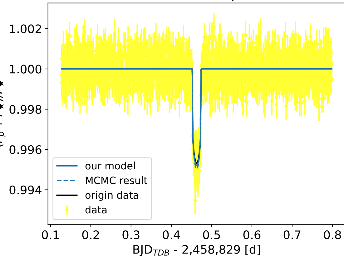
Phase curve at \lambda = 0.95 \mu\text{m} with FGS2
