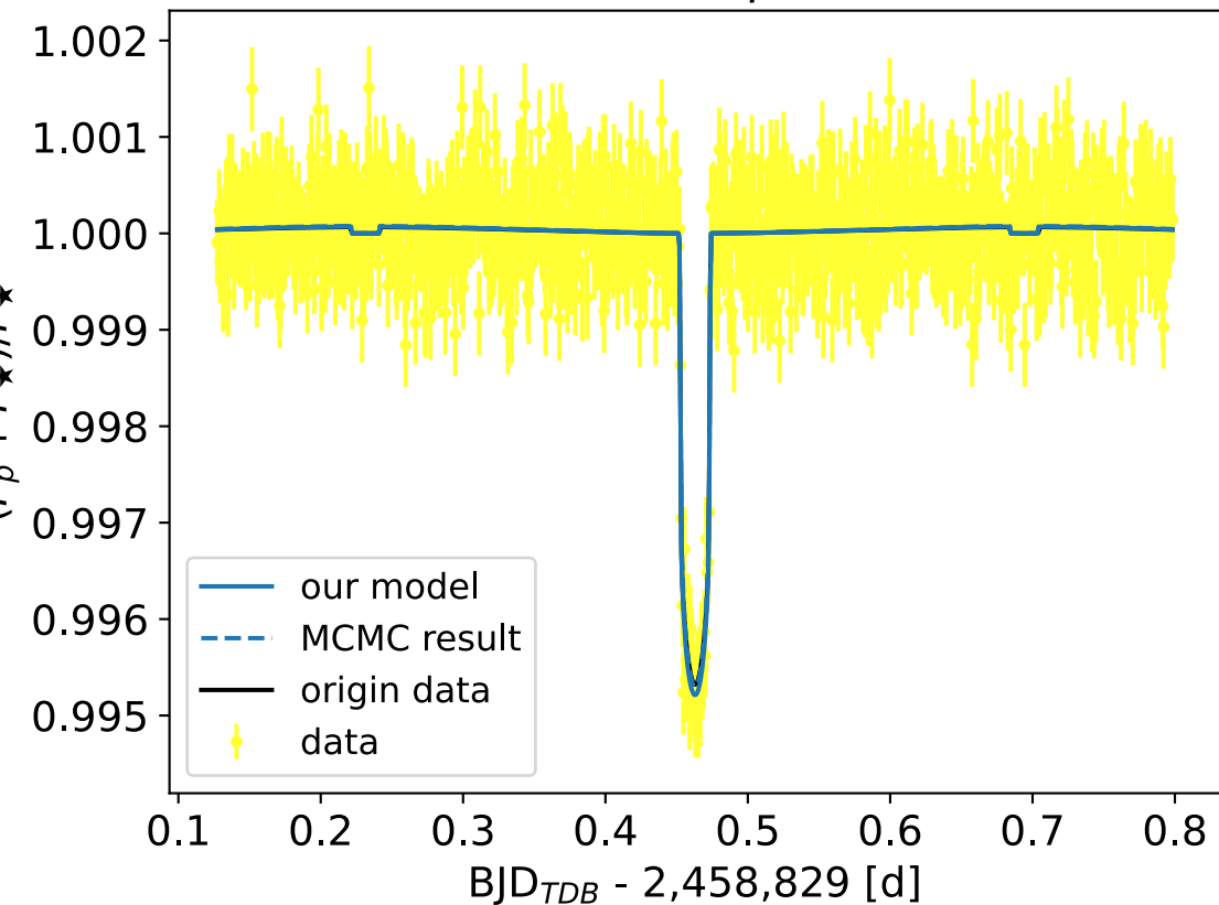
Phase curve at \lambda = 2.36 \mu\text{m} with AIRS-Ch0-1
