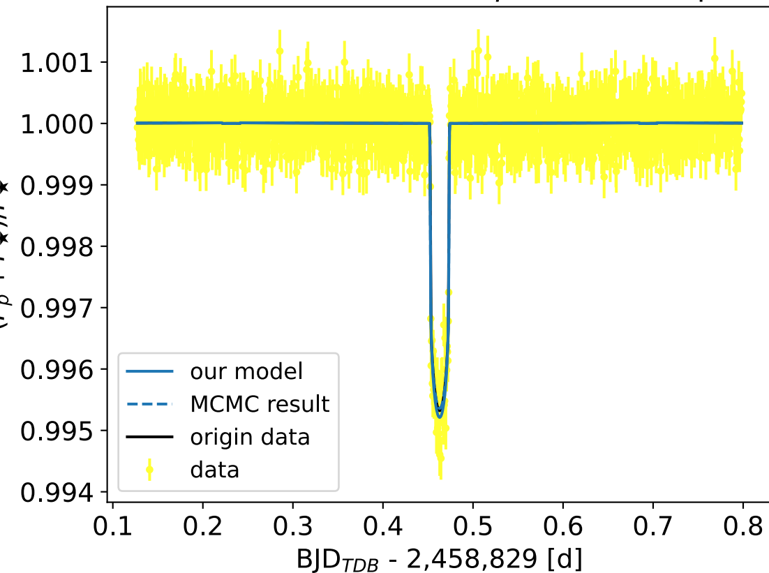
Phase curve at \lambda = 1.54 \mu\text{m} with NIRSpec
