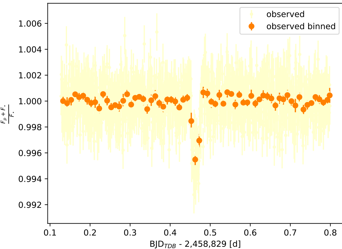
Phase curve at \lambda = 0.7 \mu\text{m} with FGS1
