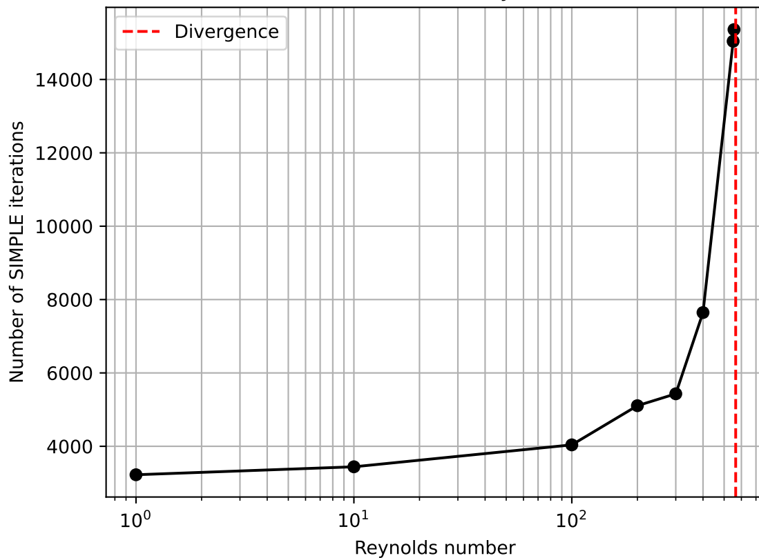
Number of iterations vs Reynolds number
