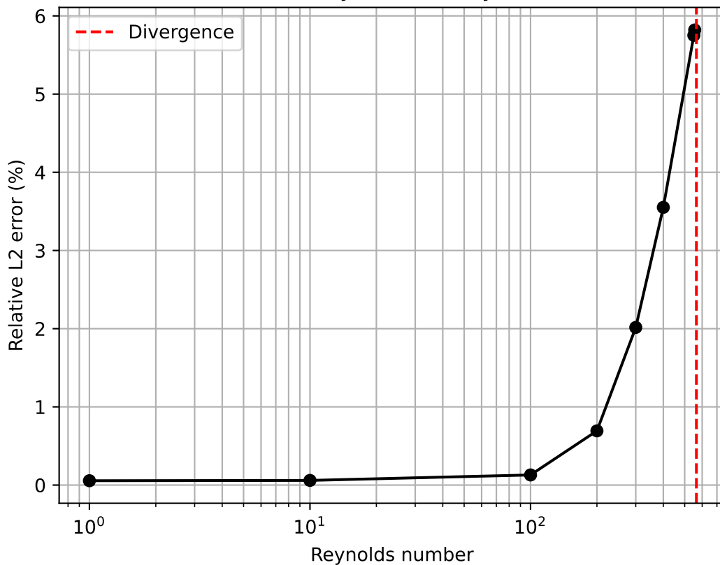
Relative L2 velocity error vs Reynolds number
