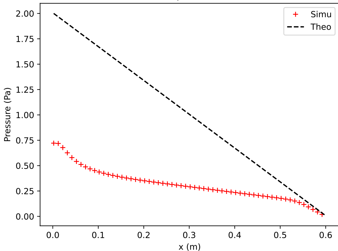
Pressure profile it= 100
