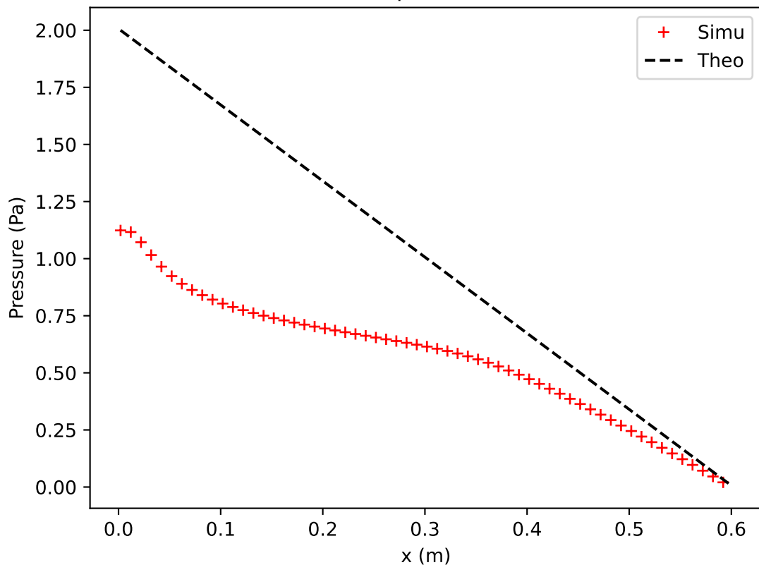
Pressure profile it= 200
