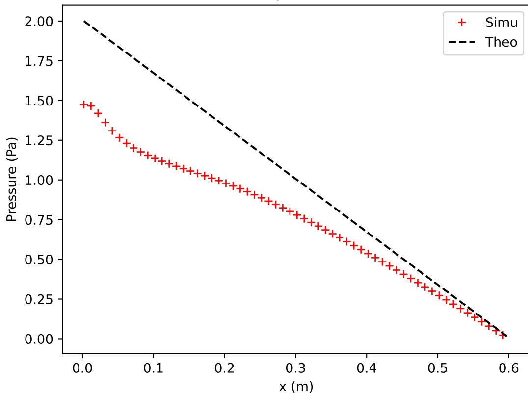
Pressure profile it= 300
