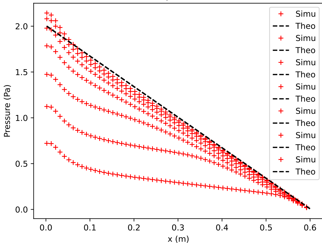
Pressure profile it= 700
