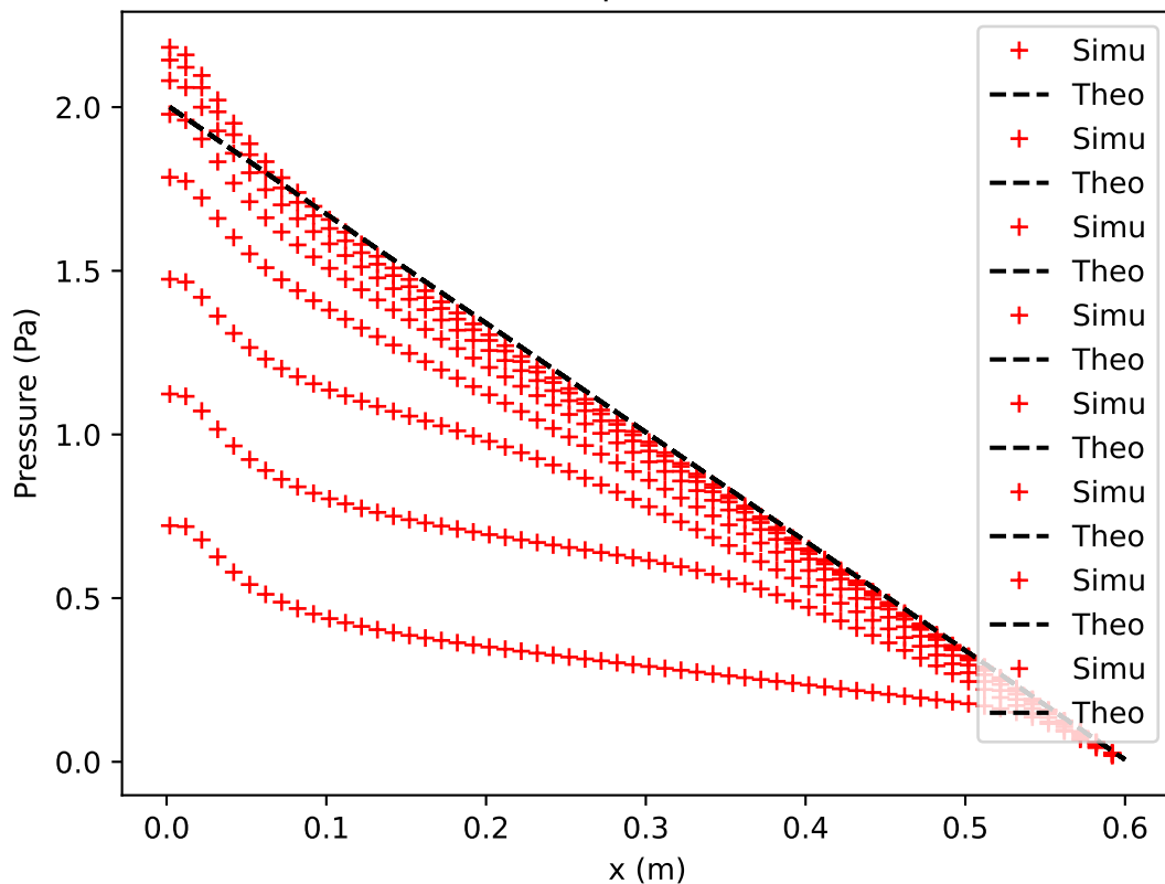
Pressure profile it= 800
