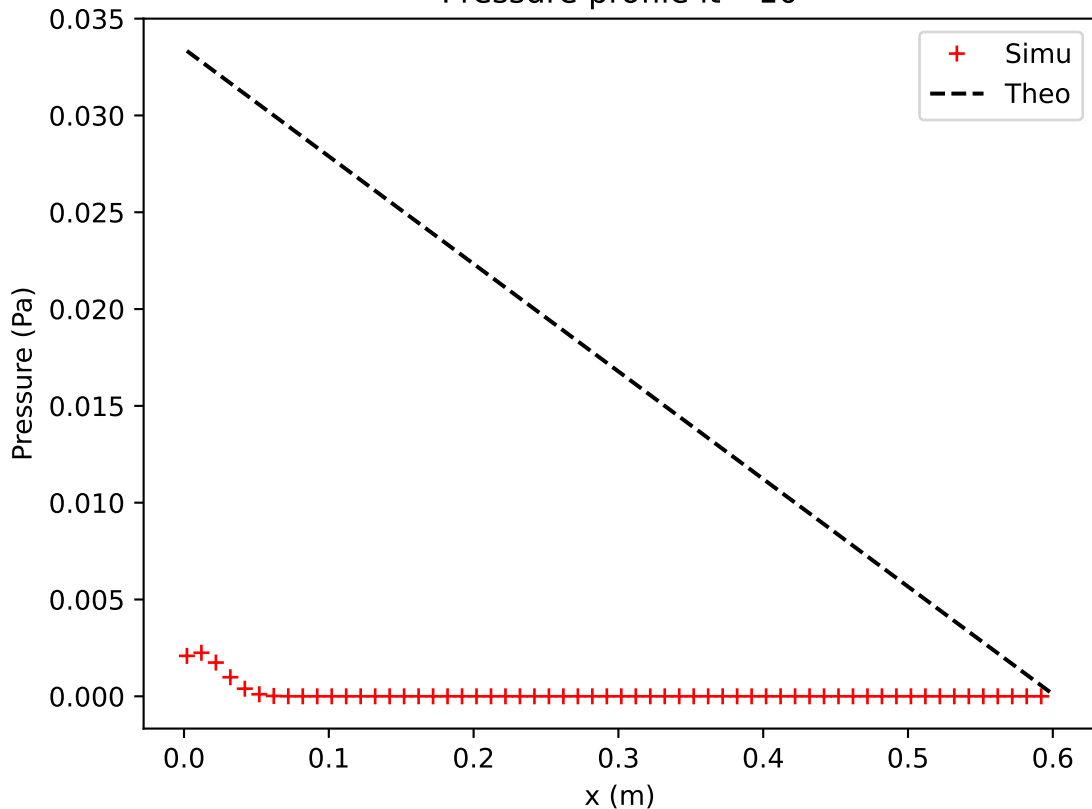
Pressure profile it= 10
